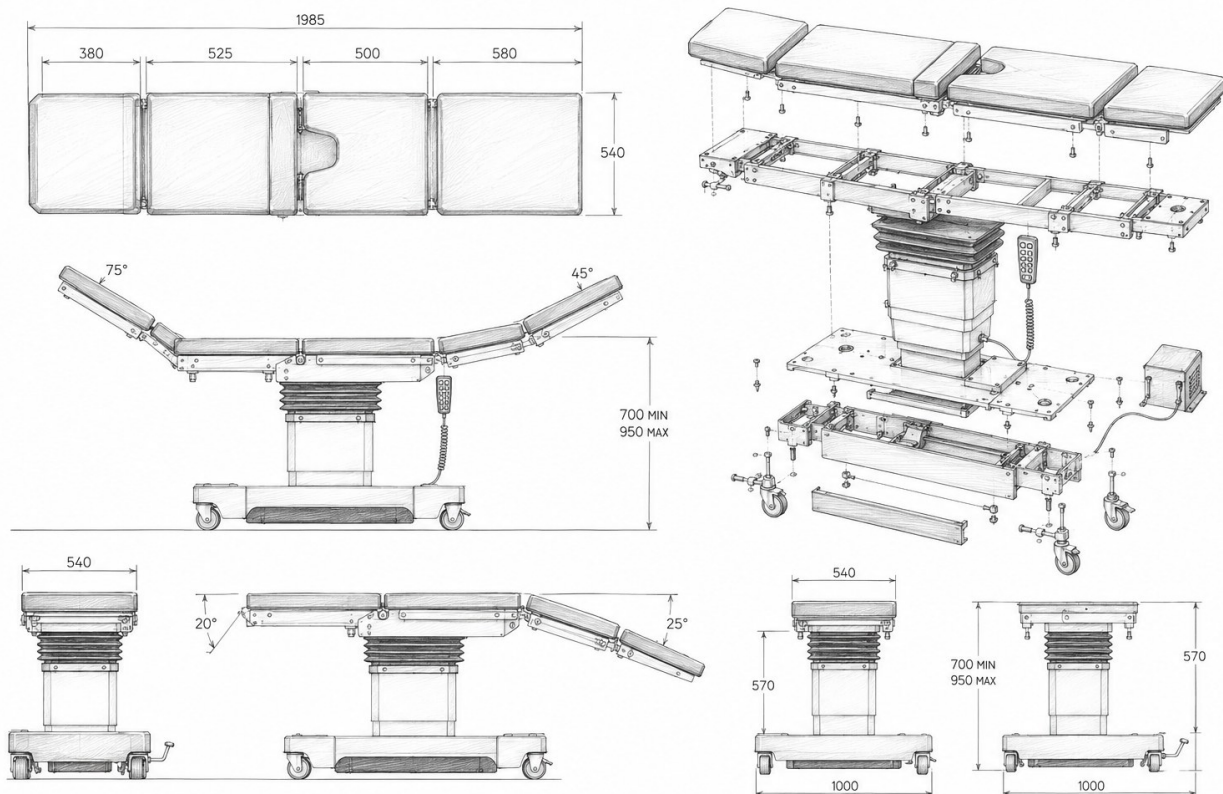
General arrangement & exploded assembly drawing – Healex 04
